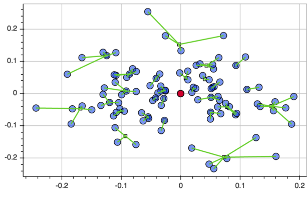
Fig. 3. Regularized geometric k -median for rideshare meetup problem. 26 ride share groups from 100 users.
