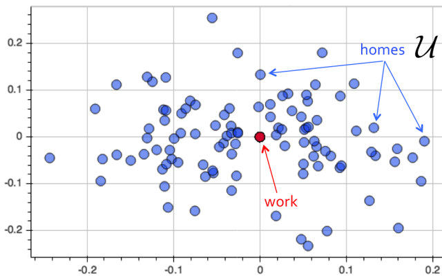
Fig. 2. Rideshare meetup problem. 100 normally distributed users, with a destination at the origin (0, 0) .
